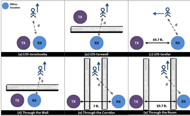
Figure 8—Scenario layouts.
